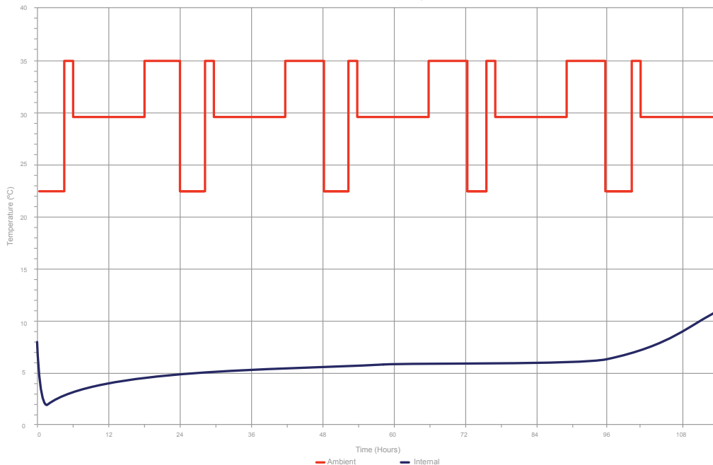
Series 4 - 2896, with Pelican Case, ISTA Summer Thermal Performance (Control Set: ISTA 7D Summer Profile, No Payload, -18°C TIC Conditioning, 23 Minute TIC Staging) Source: MTS Lab 22 February 12
